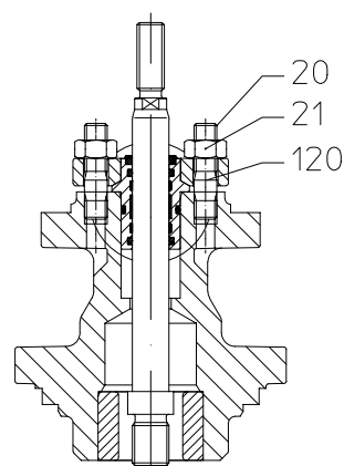
I. EPDM-sealing
